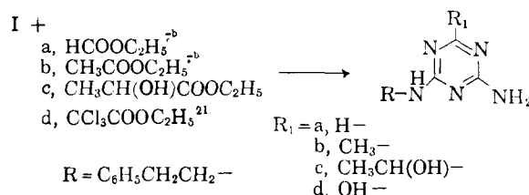
SCHEME I. REACTION OF \beta -PHENETHYLBIGUANIDE WITH ESTERS
